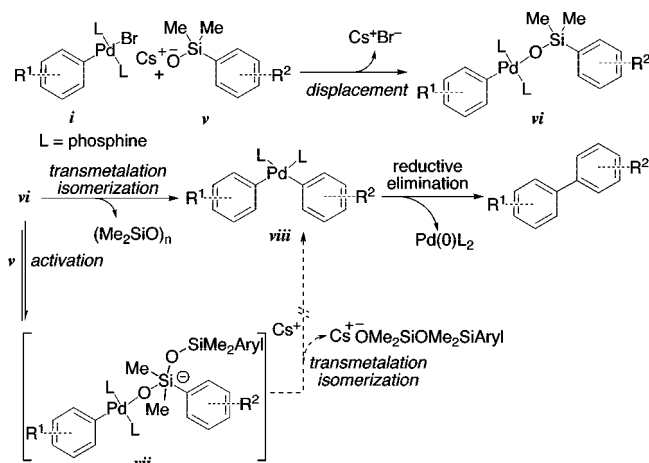
FIGURE 3. Mechanistic proposal for the coupling of aryl dimethylsilanols.
